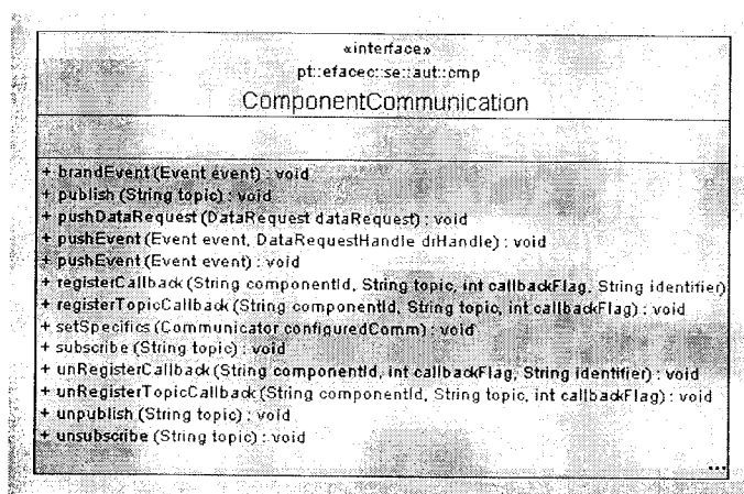
Figura 4.5: Interface ComponentCommunication
