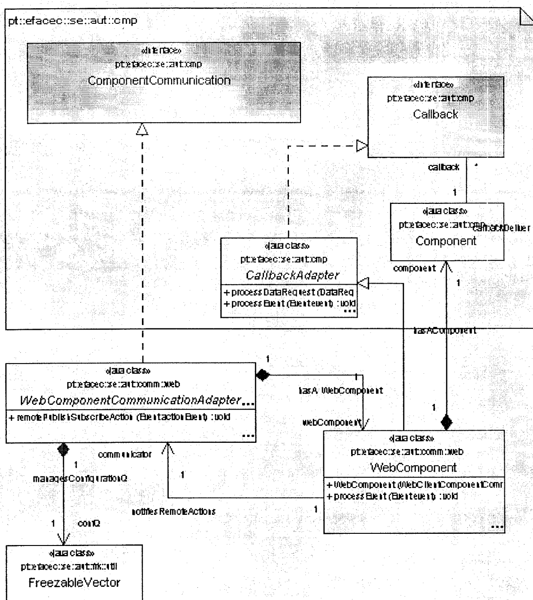
Figura 5.6: Pacote comm — Classes comuns WEB.server e WEB.client
