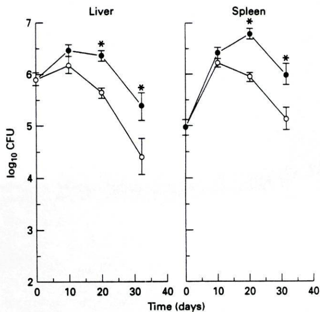
Fig. 4. Growth of Mycobacterium tuberculosis H37Ra in vivo in the spleen and liver of BALB/c animals infected with 10^6 colony-forming units (CFU) of the bacteria. Mice were treated intraperitoneally every 2 weeks with 2 mg of either anti-TNF (●) or isotype control (○) antibodies. Each time point represents the geometric mean of the CFU values from four mice \pm s.d. Statistically significant differences: * P < 0.01 .
